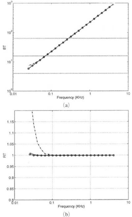
Fig. 8 The value of BT product and reverberation times calculated through EDT (---), T_{20} (—) and T_{30} (—○—) obtained using the third-octave wavelet filter bank. (a) The values of BT product, (b) Reverberation times
