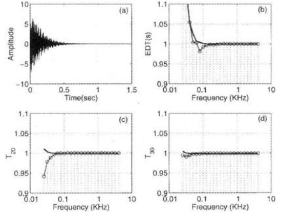
Fig. 5 Comparison between the reverberation times obtained by the third octave band wavelet filter bank (—) and the reverberation times obtained by the third octave band pass filter bank (—○—) for synthetic impulse response signal (a) Synthetic impulse response without background noise, (b) Reverberation times through EDT , (c) Reverberation times through T_{20} and (d) Reverberation times through T_{30}
