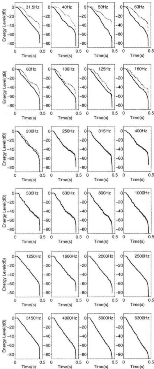
Fig. 13 Comparison between acoustic decay curves calculated with application of the third-octave band wavelet filter bank (—) and acoustic decay curves calculated with application of the third-octave band pass filter bank (·····)
