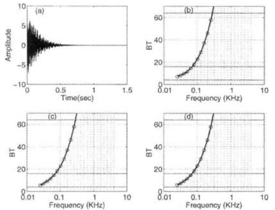
Fig. 6 Comparison between the value of BT product obtained by the third octave band wavelet filter bank (—) and the value of BT product obtained by the third octave band pass filter bank (—○—). (a) Synthetic impulse response without background noise, (b) BT product calculated through EDT , (c) BT product calculated through T_{20} and (d) BT product calculated through T_{30}
