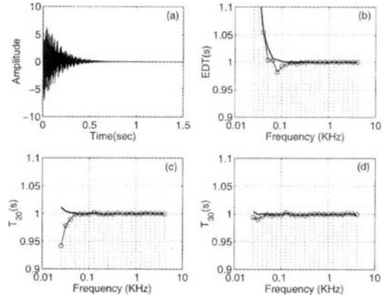
Fig. 10 Comparison between the reverberation times obtained by the third-octave band wavelet filter bank (—) and the reverberation times obtained by the third-octave band pass filter bank (—○—) for synthetic impulse response signal with background noise. (a) Synthetic impulse response with background noise. (b) Reverberation times through EDT . (c) Reverberation times through T_{20} and (d) Reverberation times through T_{30}
