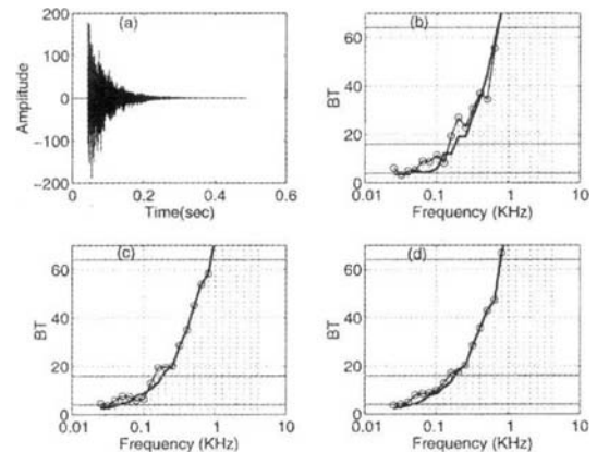
Fig. 12 Comparison between the value of BT product calculated by the third-octave band wavelet filter bank (—) and the value of BT product calculated by the third-octave band pass filter bank (—○) for the practical impulse response of the listening room for the sound quality analysis of automotive : the third-octave band wavelet filter bank. (a) Synthetic impulse response with background noise, (b) Reverberation times through EDT , (c) Reverberation times through T_{20} and (d) Reverberation times through T_{30}
